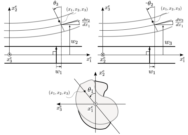
Figure 3: Deformation components in Timoshenko beam theory.
