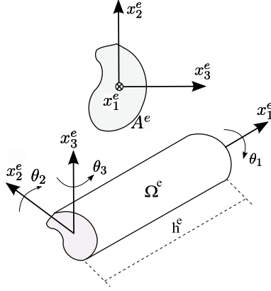
Figure 2: 3D beam local coordinates.
