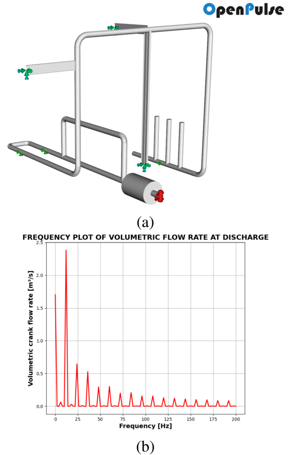
Figure 7: (a) Simple example of a piping system supported by “I” type beams. In red: discharge of a reciprocating compressor. In green: displacement constraints. (b) Frequency plot of volumetric flow rate at the discharge of a compressor.
