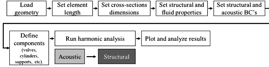
Figure 5: Sequence of problem set-up in OpenPulse .
