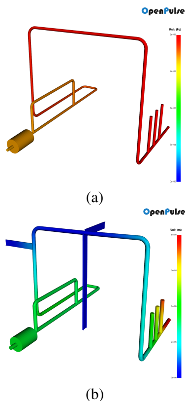
Figure 8: (a) Acoustic response and (b) structural response at 12 Hz. Colormap: amplitudes.
