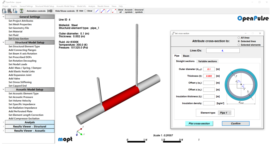
Figure 6: Main window of OpenPulse . Entry of properties and section parameters.
