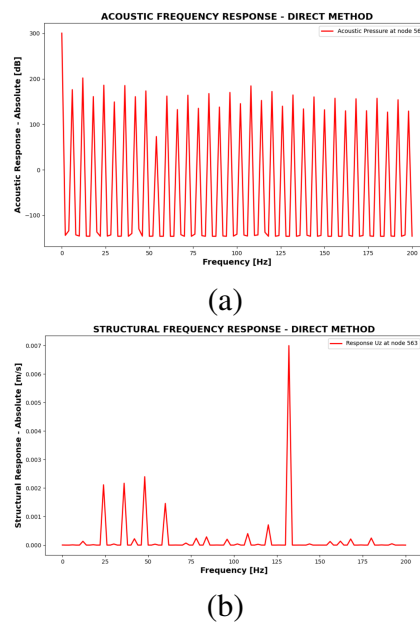
Figure 9: (a) Frequency plot of pressure amplitude and (b) x-velocity amplitude at node 563.
