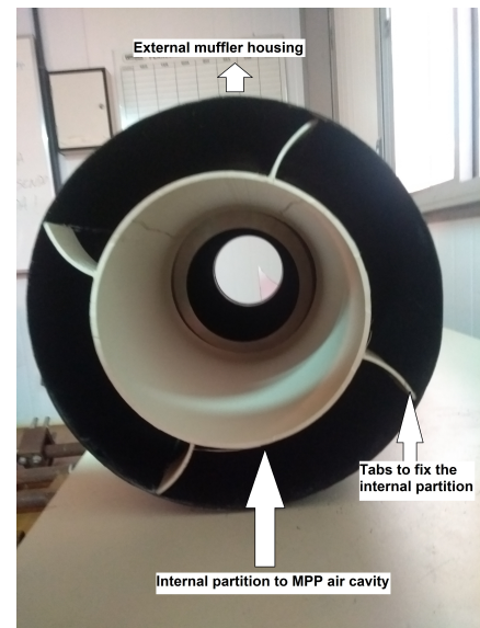
Figure 12: Muffler with internal partitions in the MPP air cavity depth.
