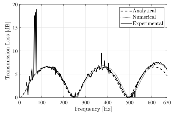
Figure 6: Comparison between the three TL curves for a simple expansion chamber model.
