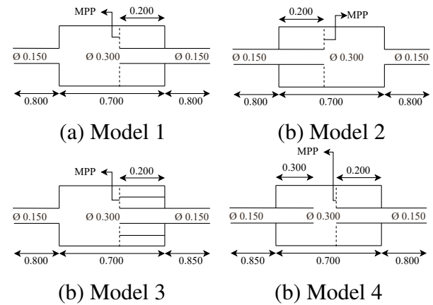
Figure 2: Models of ECAF-MPP.
