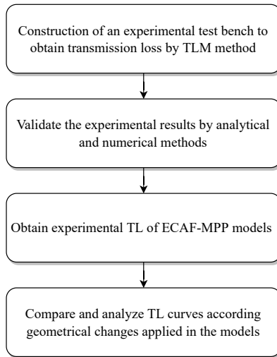
Figure 1: Summary flowchart of the methodology.
