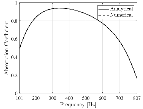
Figure 9: Absorption coefficient of MPP with air cavity depth of L_2 .
