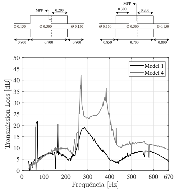
Figure 14: Comparisons of TL of models 1 and 4.
