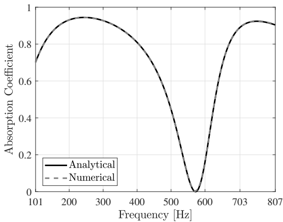
Figure 8: Absorption coefficient of MPP with air cavity depth of L_1 .
