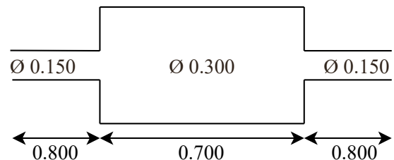
Figure 3: Simple expansion chamber model (SEC).
