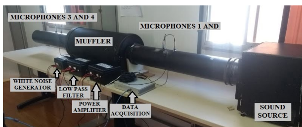
Figure 5: Experimental test bench constructed to measure TL of ECAF-MPP models.
