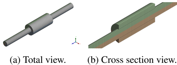
Figure 4: Numerical model of SEC in ANSYS®.
