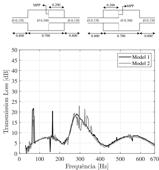
Figure 11: Comparison of TL of models 1 and 2.
